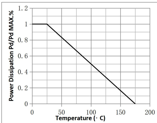
Fig.1 Power Dissipation
