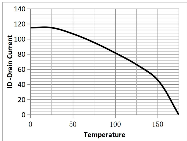
Fig.12 I_D -Junction Temperature
