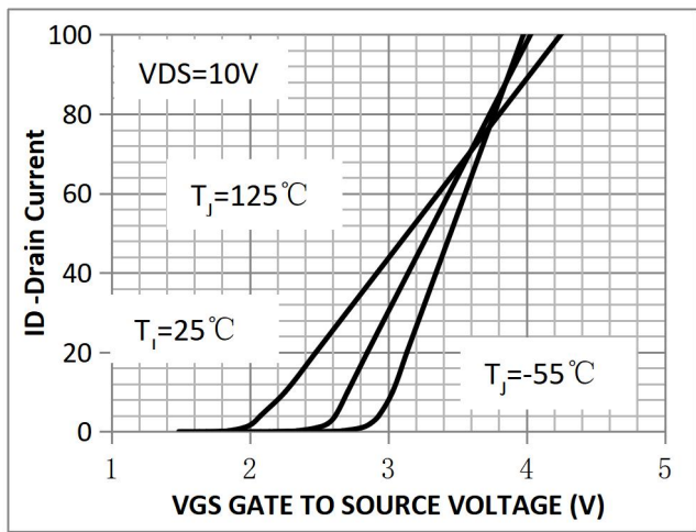
Figure 10. Transfer Characteristics
